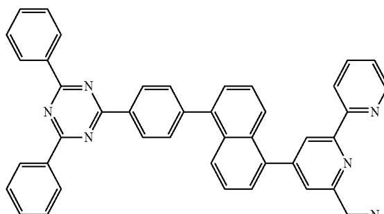
[Chemical Formula 5]
