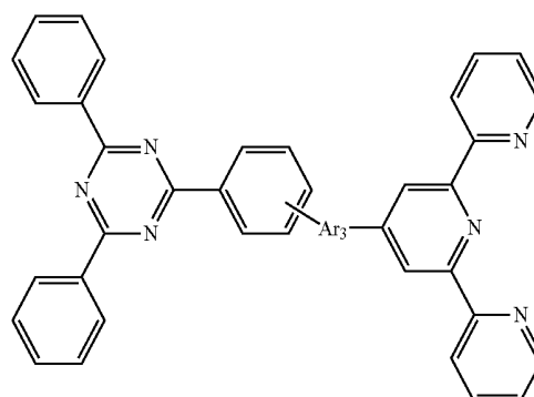
[Chemical Formula 2]
