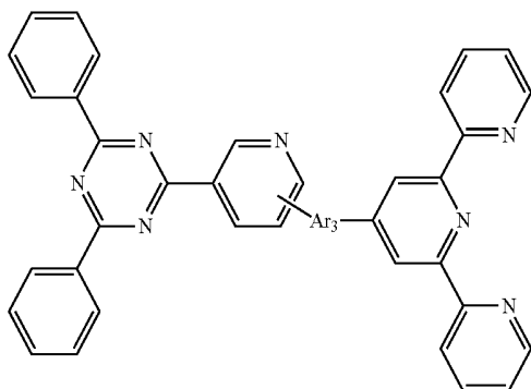
[Chemical Formula 3]
