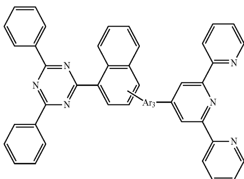
[Chemical Formula 5]
